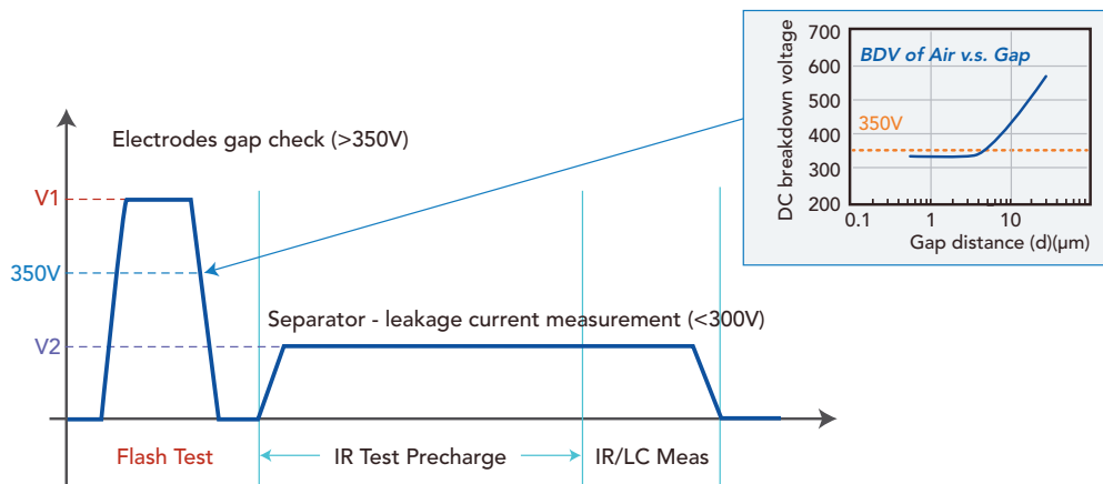
[Figure 9] Application of Chroma 11210 + Flash Test function during inspection of Li-ion Battery insulation quality
