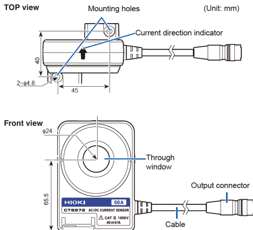
Figure 5. Dimensions
