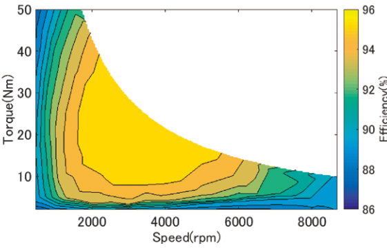
Example of an efficiency map display in MATLAB
