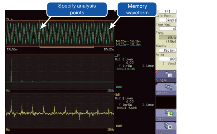
Display the calculation source (memory waveform) and FFT calculation results at the same time
