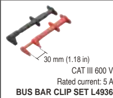
BUS BAR CLIP SET L4936
