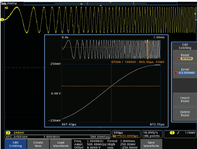
Arbitrary waveform editor showing the point-by-point editor.
