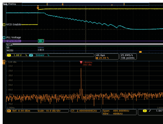
3. Spectrum Time is moved another 160 \mu s to the right. At this point the spectrum shows that the PLL has actually overshot the correct frequency and gone all the way down to 2.3888 GHz.
