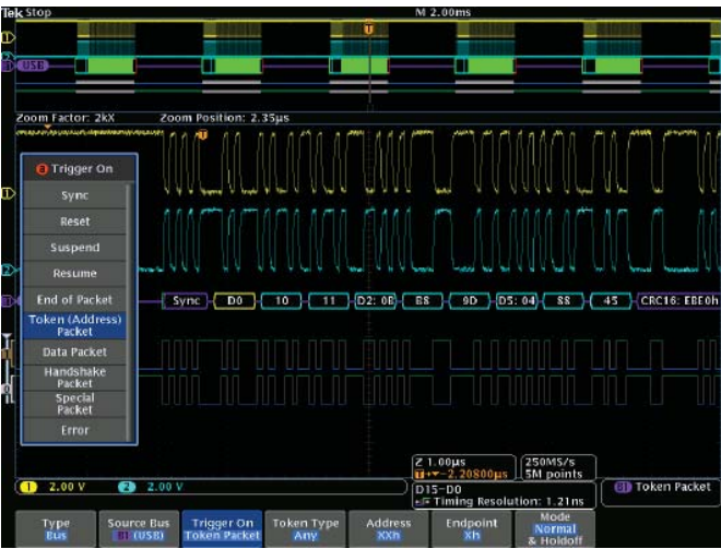
Triggering on a specific OUT Token packet on a USB full-speed serial bus. The yellow waveform is the D+ and the blue waveform is the D-. A bus waveform provides decoded packet content including Start, Sync, PID, Address, End Point, CRC, Data values, and Stop.
