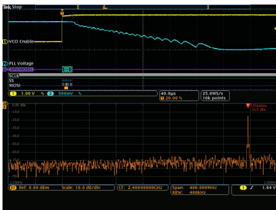
1. Time and Frequency Domain view showing the turn-on of a PLL. Channel 1 (yellow) is probing a control signal that enables the VCO. Channel 2 (cyan) is probing the VCO tune voltage. The SPI bus which is programming the PLL with the desired frequency is probed with three digital channels and automatically decoded. Notice Spectrum Time is placed after the VCO was enabled and coincident with the command on the SPI bus telling the PLL the desired frequency of 2.400 GHz. Note that the RF is at 2.5564 GHz when the circuit turns on.
