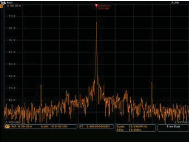
MDO4000C frequency domain display.
