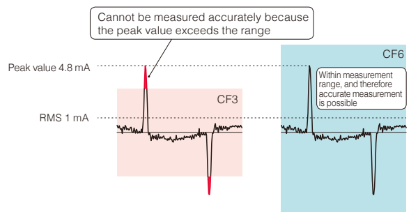
Example of Standby Current Waveform (CF = Peak Value, RMS = 4.8)
